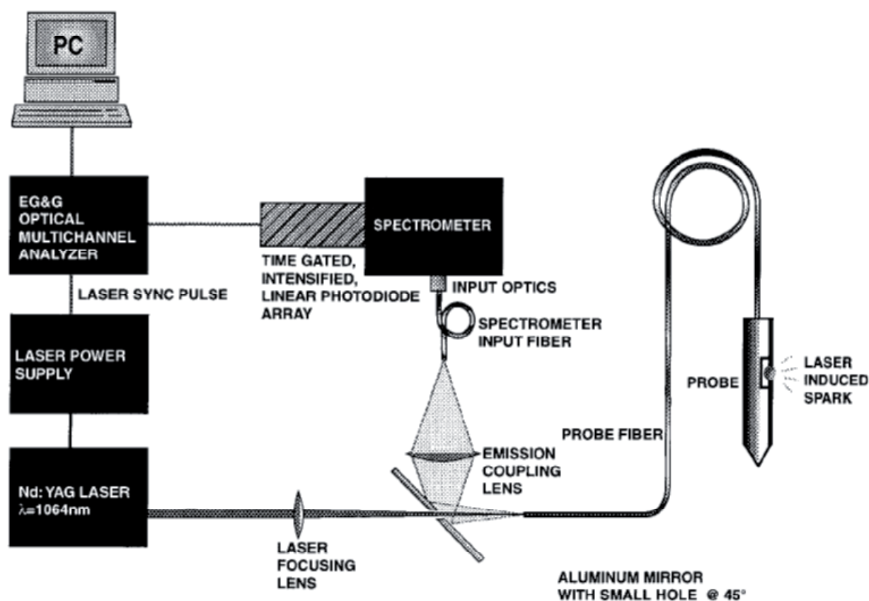
Figure 19: Schematic of the LIBS set up (Theirault et al, 1998).
