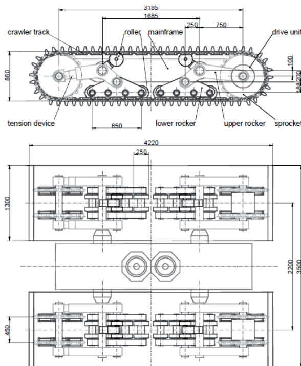
Figure 35: A crawler chassis design (Wenzlawski, 2000)
